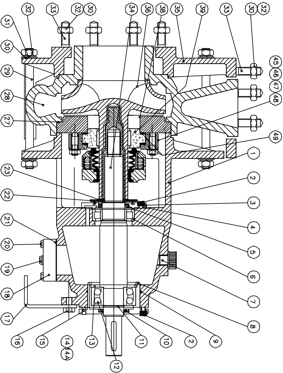
TYPICAL ASSEMBLY OF KSI GROUP II MODEL PUMPS FITTED WITH JOHN CRANE 10T/10R TYPE MECHANICAL SHAFT SEALS.
