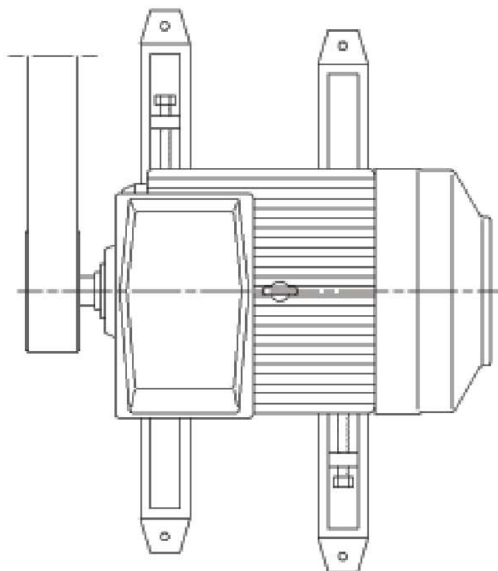
Figure 2. Belt drive
